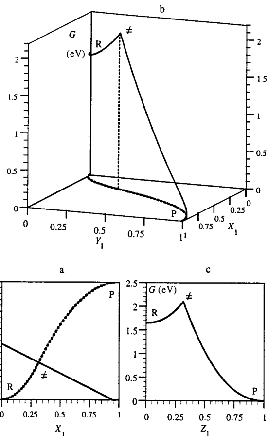
Figure 1. RX \pm e^- \leftrightarrow R^\bullet + X^\mp . In electronvolts, D = 3 , \lambda_{0,1} = 1.5 , G_{RX\pm e^-}^0 = 1.65 , G_{R^\bullet+X^\mp}^0 = 0 . (a) Full line: projection of the intersection of the two surfaces 1 and 2, dotted line: projection of the steepest descent pathway. (b) Steepest descent reaction pathway. (c) Steepest descent reaction profile as a function of the reaction coordinate Z_1 . R: RX \pm e^- , P: R^\bullet + X^\mp .
