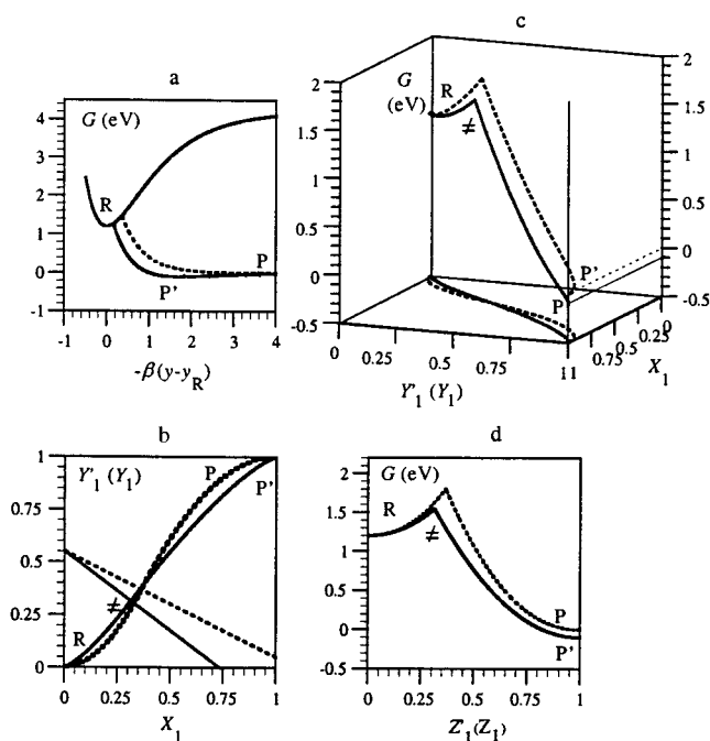
Figure 5. Influence of a small interaction between caged fragments. Full lines: \text{RX} \pm \text{e}^- \rightleftharpoons (\text{R}\cdot, \text{X}^\mp) . Dotted lines: \text{RX} \pm \text{e}^- \rightleftharpoons \text{R}\cdot + \text{X}^\mp . In eV, D = 3 , \lambda_{0,1} = 1.5 , D_{\text{p}} = 0.1 , G_{\text{RX}\pm\text{e}^-}^0 = 1.65 , G_{\text{R}\cdot + \text{X}^\mp}^0 = 0 , G_{(\text{R}\cdot, \text{X}^\mp)}^0 = -0.1 . (a) Morse curves for the reactant, interacting fragments and separated fragments. (b) Projection of the reaction pathways on the X_1 - Y_1 plane. (c) Reaction profiles as a function of the reaction coordinate Z_1 or Z_1 . R: \text{RX} \pm \text{e}^- , P: \text{R}\cdot + \text{X}^\mp , P': (\text{R}\cdot, \text{X}^\mp) . (d) Steepest descent reaction profile as a function of the reaction coordinate Z_1 or Z_1 .
