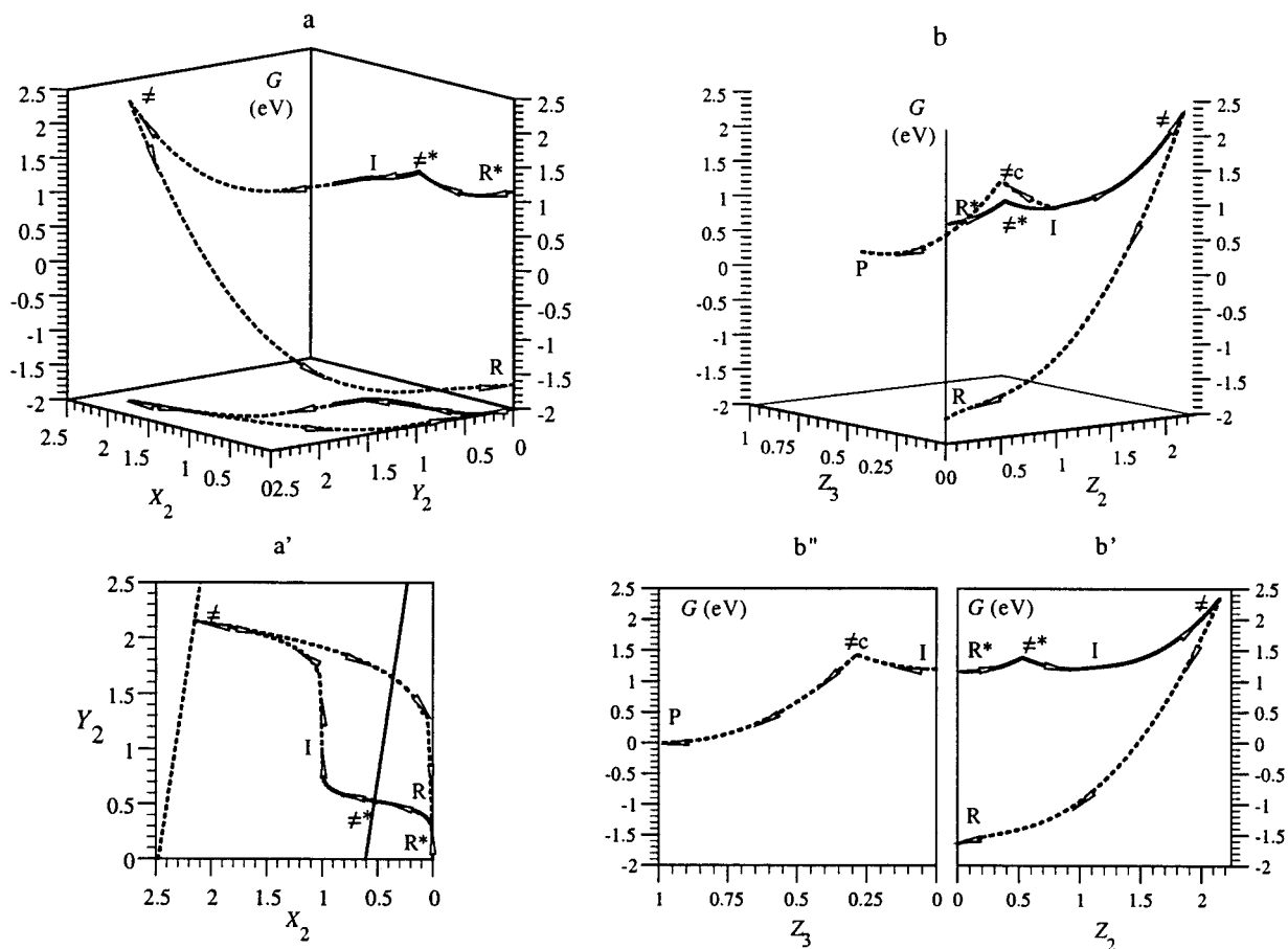
Figure 3. Reaction pathway for a photoinduced reaction following a stepwise mechanism in which the electron transfer is in the inverted region. In eV, G_{D^+ + RX}^0 = 1.15 , G_{D^+ + RX}^* = -1.65 , G_{D^+ + RX^-}^0 = 1.2 , G_{D^+ + R^+ + X^-}^0 = 0 , (\sqrt{D} - \sqrt{D'})^2 = 0.1 , D' = 1.8 , \lambda_{0,2} = 0.75 , \lambda_{0,3} = 1 . R*: D^+ + RX , R: D + RX , I: D^+ + RX^* , P: D^+ + R^+ + X^- . \neq^* , \neq , \neq_c , transition states of the photoinduced electron transfer, back electron transfer, and cleavage, respectively.
