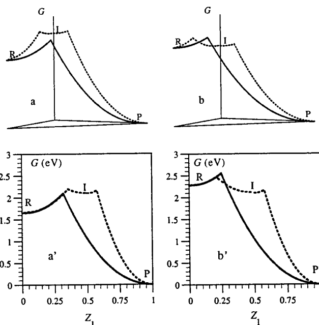
Figure 2. 3-dimensional (a, b) and 2-dimensional (a', b') representations of the concerted (full line) and stepwise (dotted lines) reaction pathways. \text{RX} \pm e^- \leftrightarrow \text{R}^{\cdot} + \text{X}^{\mp} : D = 3 eV, \lambda_{0,1} = 1.5 eV, G_{\text{RX}}^0 = 1.65 eV (left-hand diagrams), 2.28 eV (right-hand diagrams). \text{RX} \pm e^- \leftrightarrow \text{RX}^{\pm} : (\sqrt{D} - \sqrt{D'})^2 = 0.1 eV, \lambda_{0,2} = 1 eV, G_{\text{RX}^{\pm}}^0 = 2.1 eV. \text{RX}^{\pm} \leftrightarrow \text{R}^{\cdot} + \text{X}^{\mp} : D' = 2 eV, \lambda_{0,3} = 1 eV, G_{\text{R}^{\cdot} + \text{X}^{\mp}}^0 = 0 . R: reactants ( \text{RX} \pm e^- ), I: intermediate ( \text{RX}^{\pm} ), P: products ( \text{R}^{\cdot} + \text{X}^{\mp} ).
